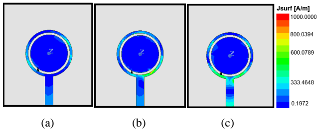
Fig. 5. Current density of antenna when diode is off: (a) 3.02 GHz, (b) 3.66 GHz, (c) 6.47 GHz
