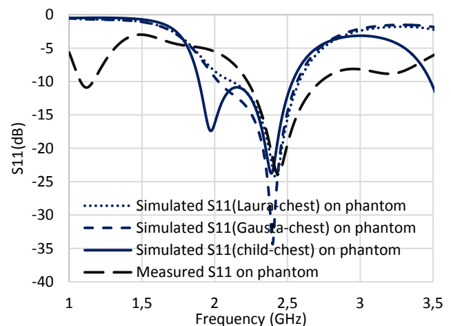
Fig. 13. Simulated Reflection coefficient the wearable button DRA for different phantom which has been placed on the chest and also measured on phantom.
