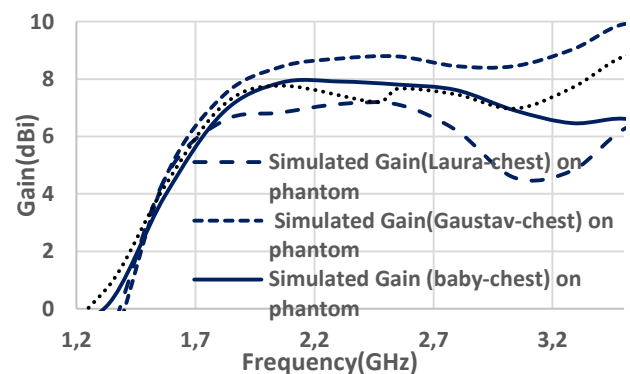
Fig. 14. Simulated Gain of the wearable button DRA for different phantom which has been placed on the chest and also measured on phantom.
