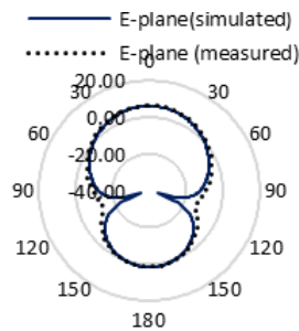
Fig. 11. Simulated and measured Radiation pattern in E-plane
