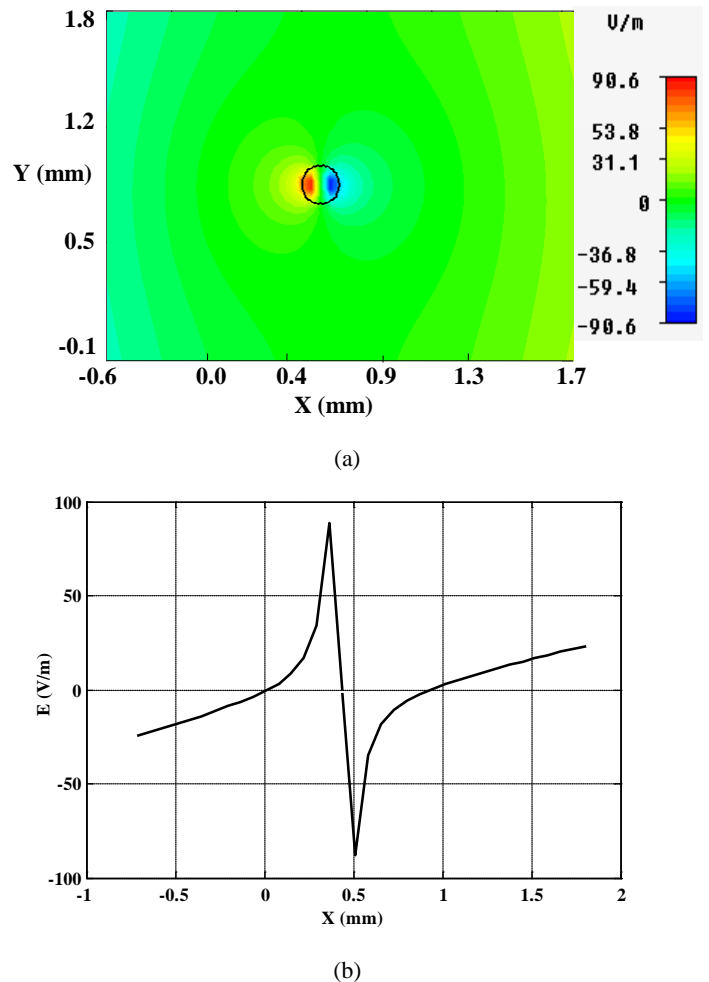
Fig. 7. E field distribution inside the single pollen (a) at XY plane for Z = 0 and (b) along the X-axis
