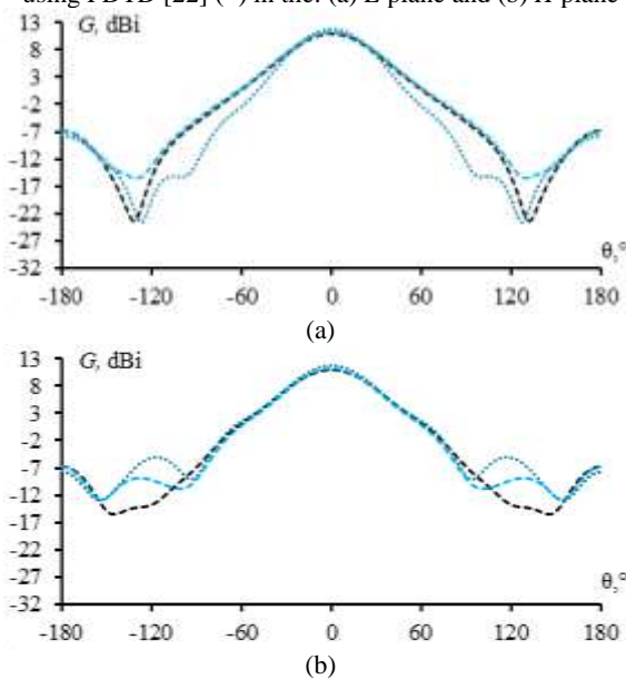
Fig. 10. Conical horn AGs for structures obtained using OCGA with GEET of 6% (···) and 10% (---) and those obtained using COCGA with GEET of 6% (···) and 10% (---) in the: (a) E plane and (b) H plane
