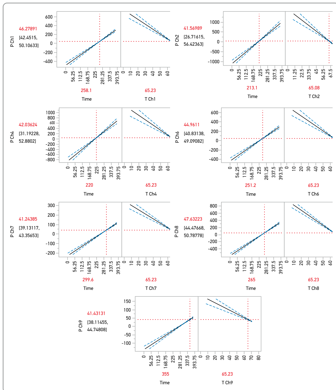
Figure 7. Prediction of pasteurisation time necessary to achieve a P0 value >40 at approximately 65oC
