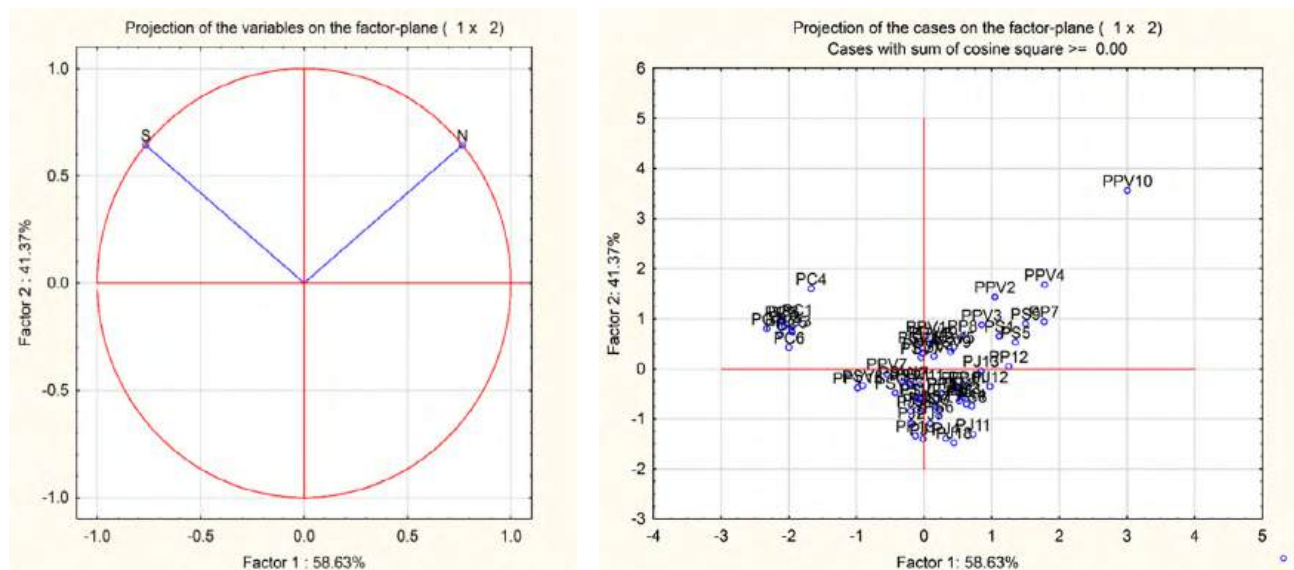
Figure 1 a). PCA loading plot in the plane of factors 1 and 2 – the labels correspond to sodium chloride (S) and nitrite (N) content. b) PCA score plot in the plane of factors 1 and 2 – the labels correspond to the meat products given in materials and methods.
