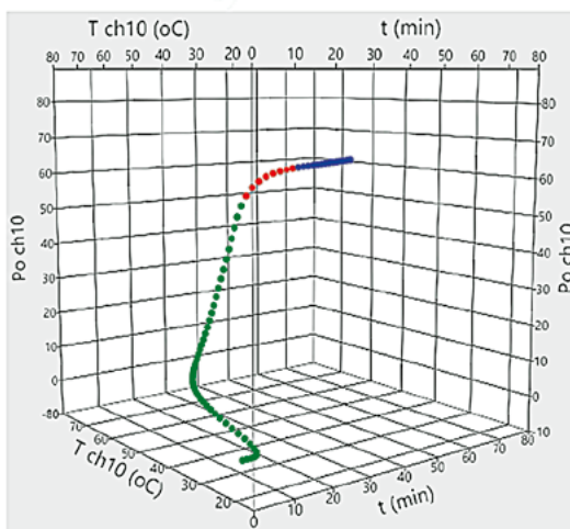
Figure 4. 3D scatter plots of pv value vs time and temperature in sausage centers as recorded by thermocouple probe channels: a) channel 2; b) channel 4; c) channel 5; d) channel 7; e) channel 8; f) channel 10; g) channel 11. Colors of data points correspond to the colors in Table 1
